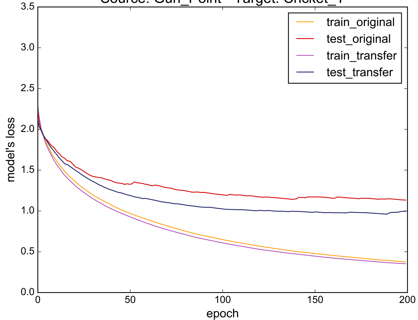
Source: Gun_Point - Target: Cricket_Y
