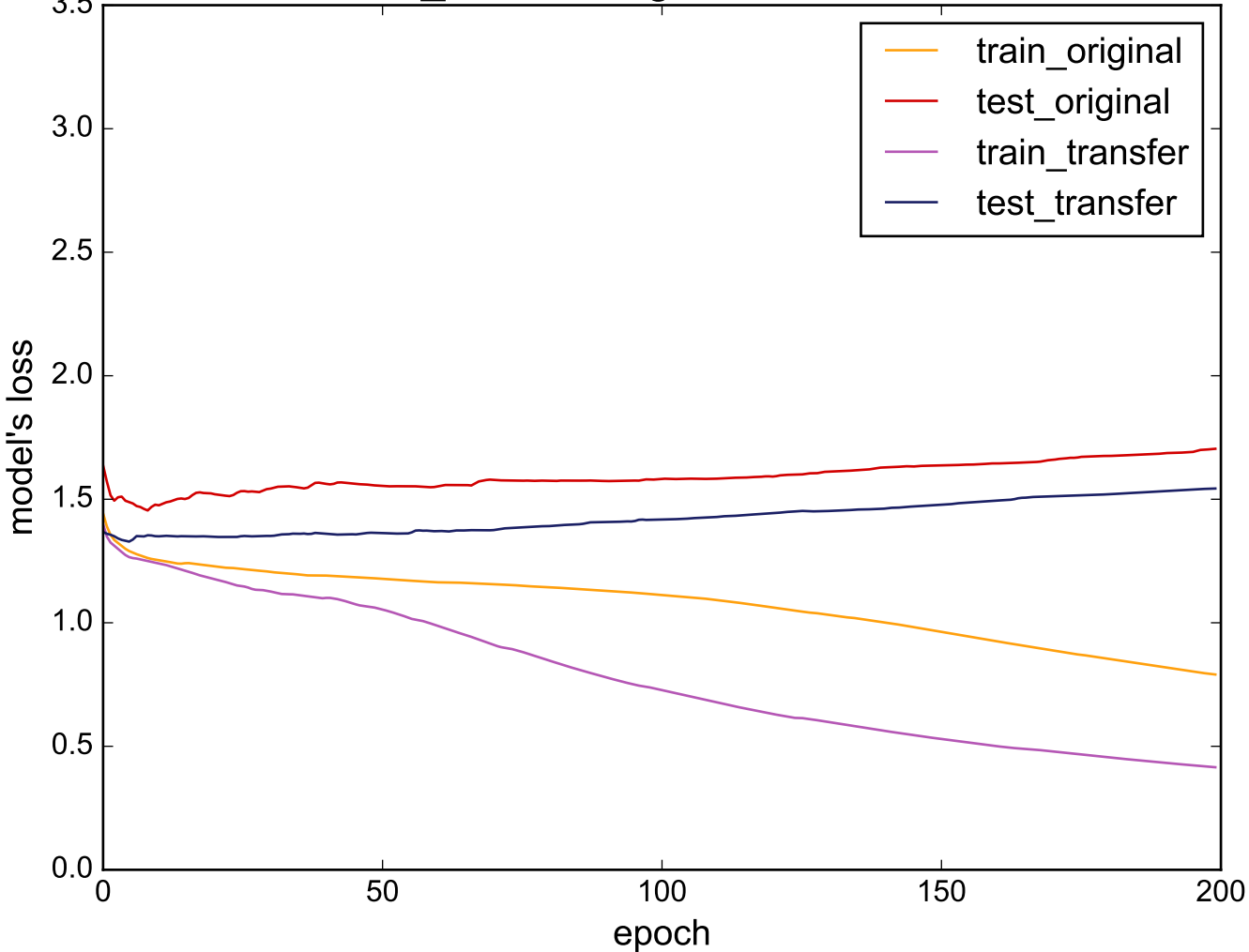
Source: Gun_Point - Target: DiatomSizeReduction
