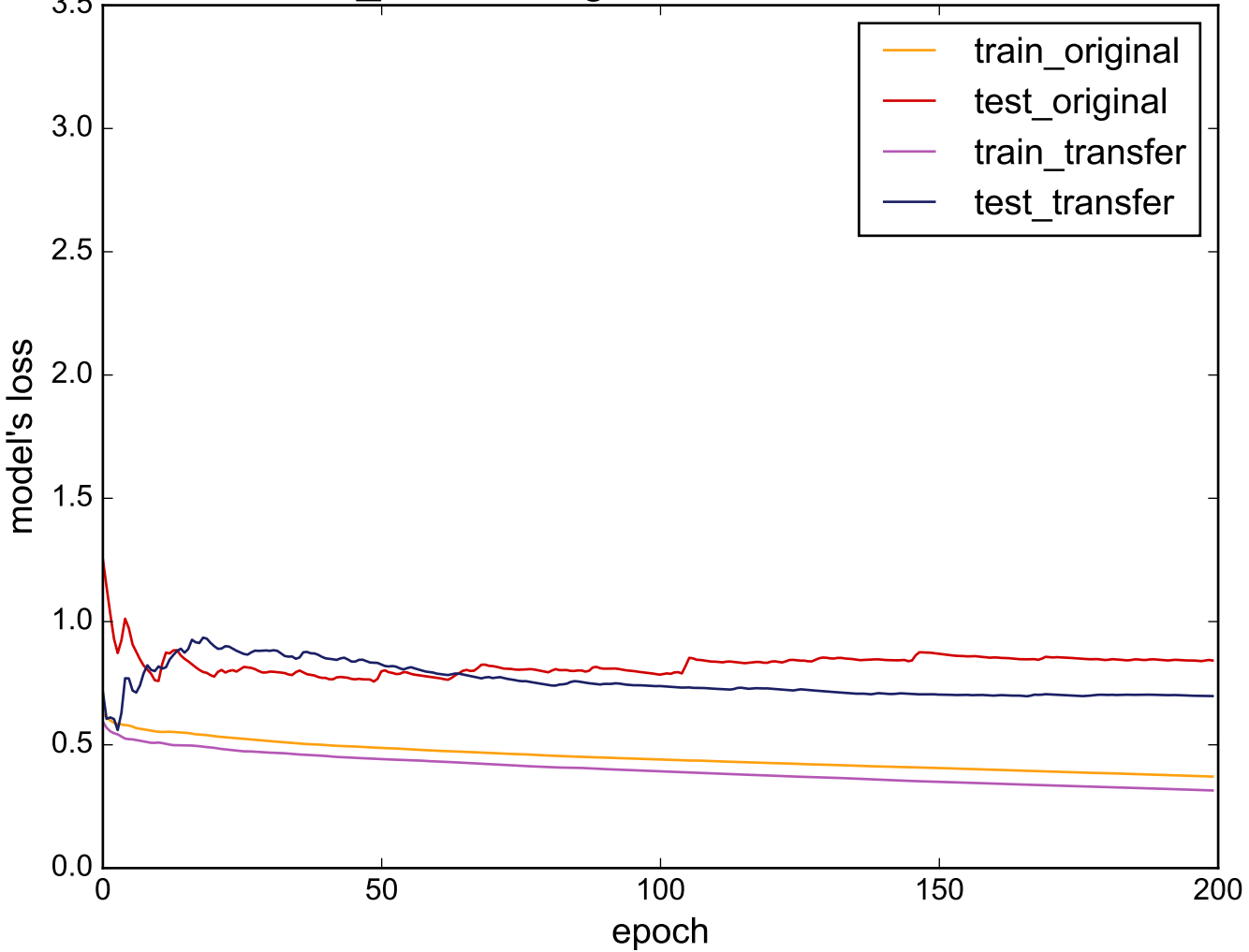
Source: Gun_Point - Target: DistalPhalanxOutlineCorrect
