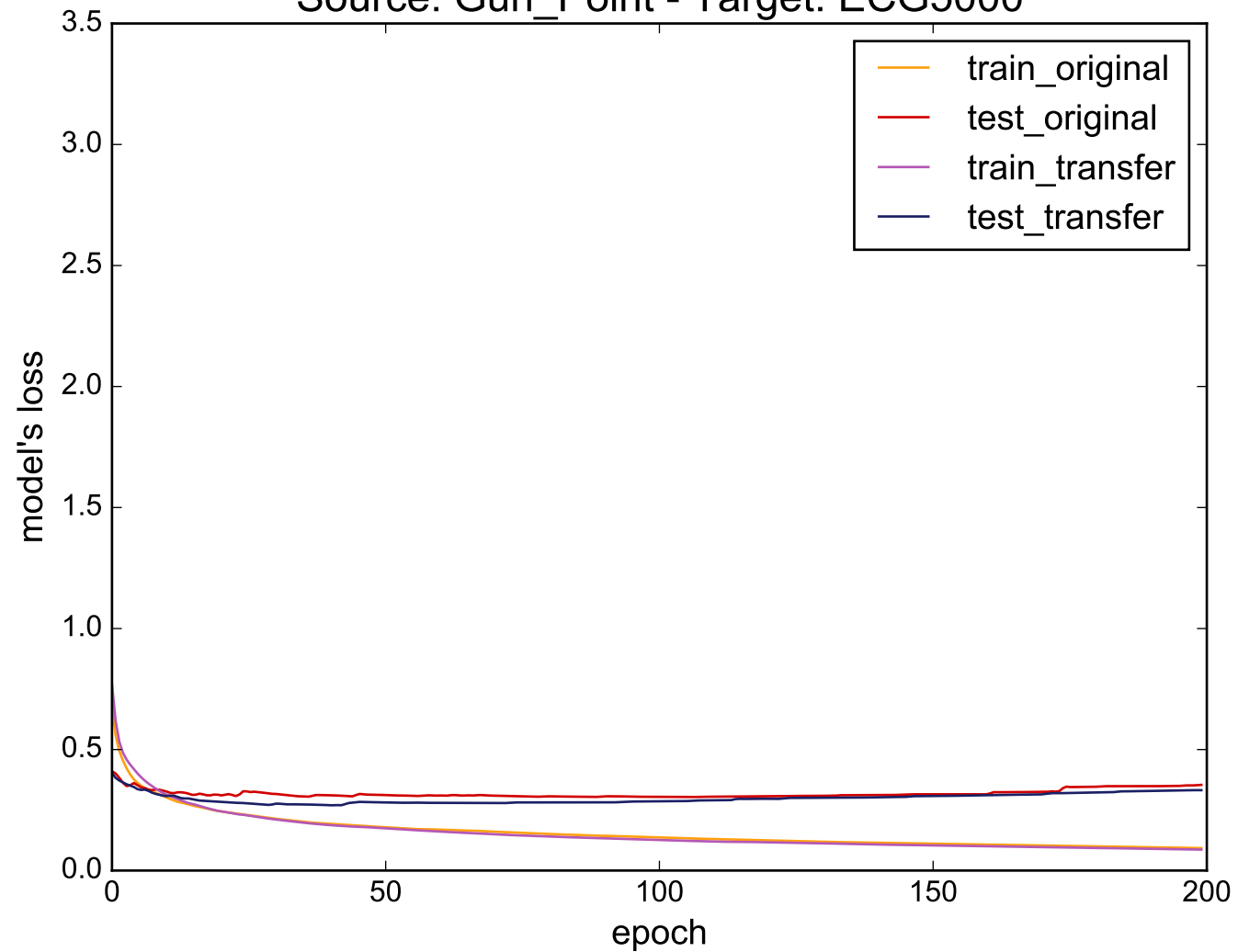
Source: Gun_Point - Target: ECG5000
