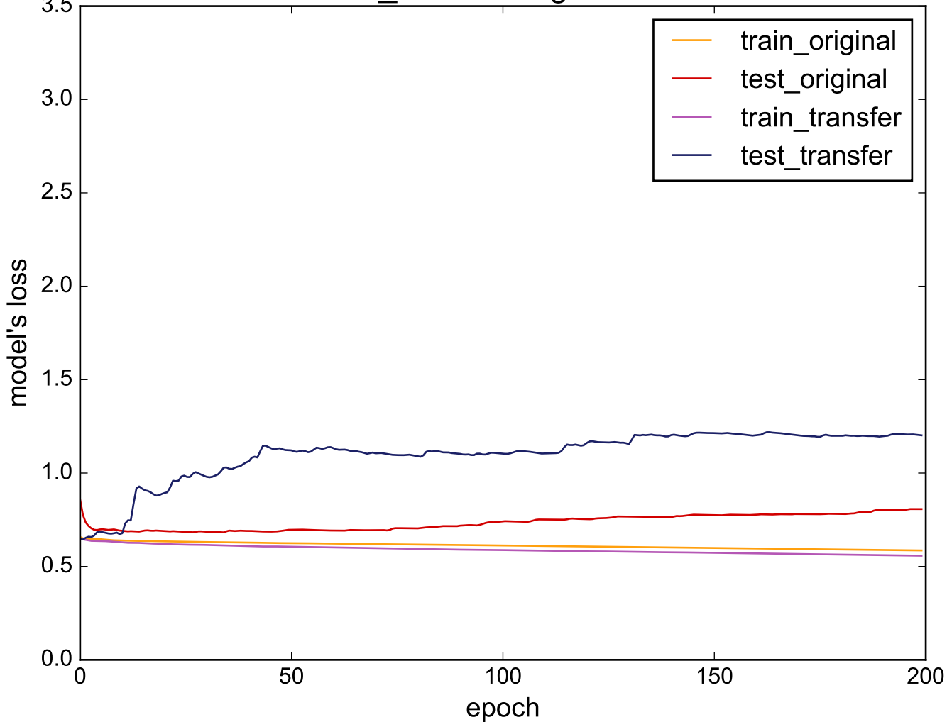
Source: Gun_Point - Target: HandOutlines
