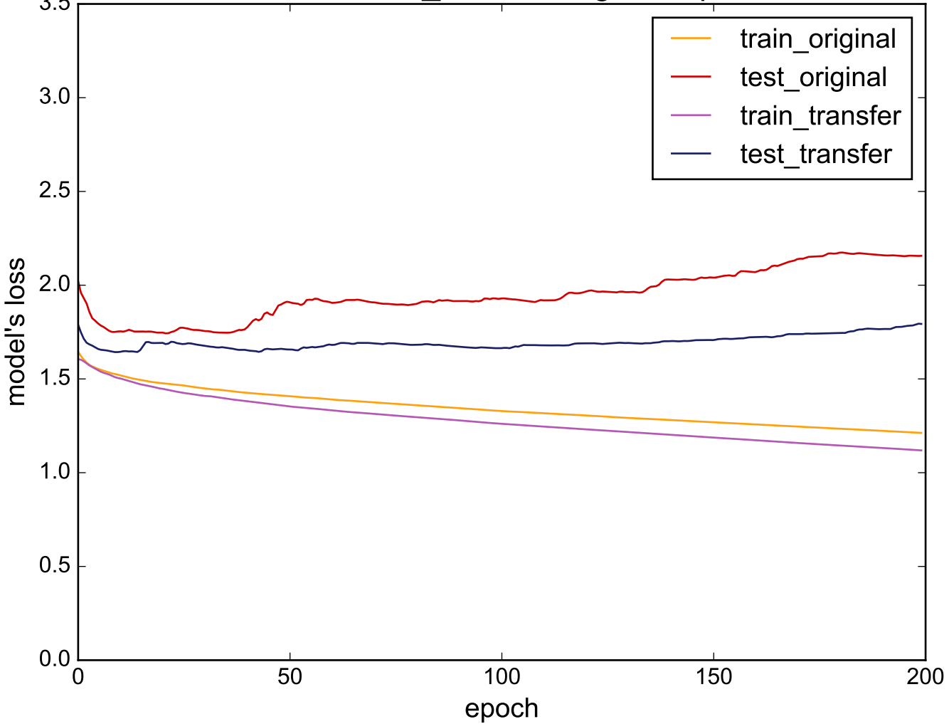
Source: Gun_Point - Target: Haptics
