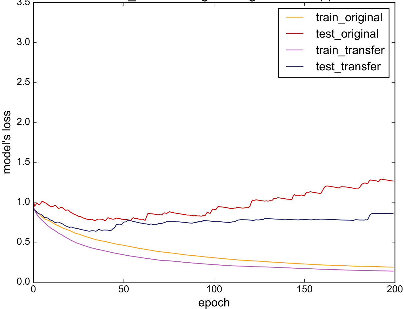
Source: Gun_Point - Target: LargeKitchenAppliances
