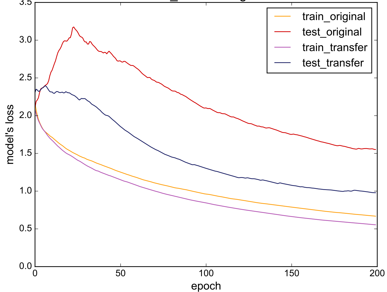
Source: Gun_Point - Target: MALLAT
