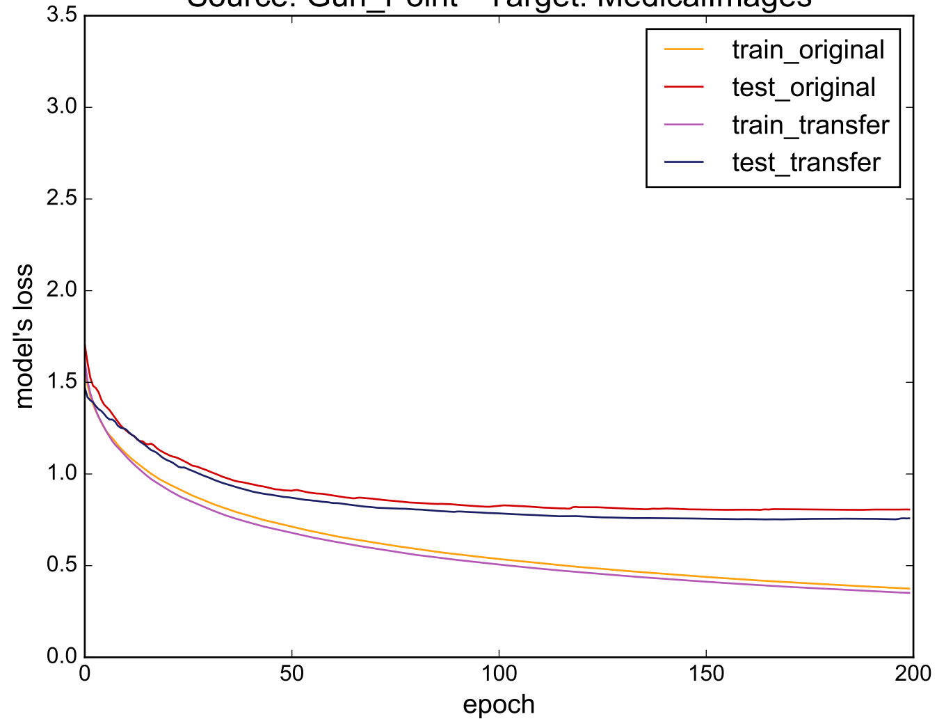
Source: Gun_Point - Target: MedicalImages
