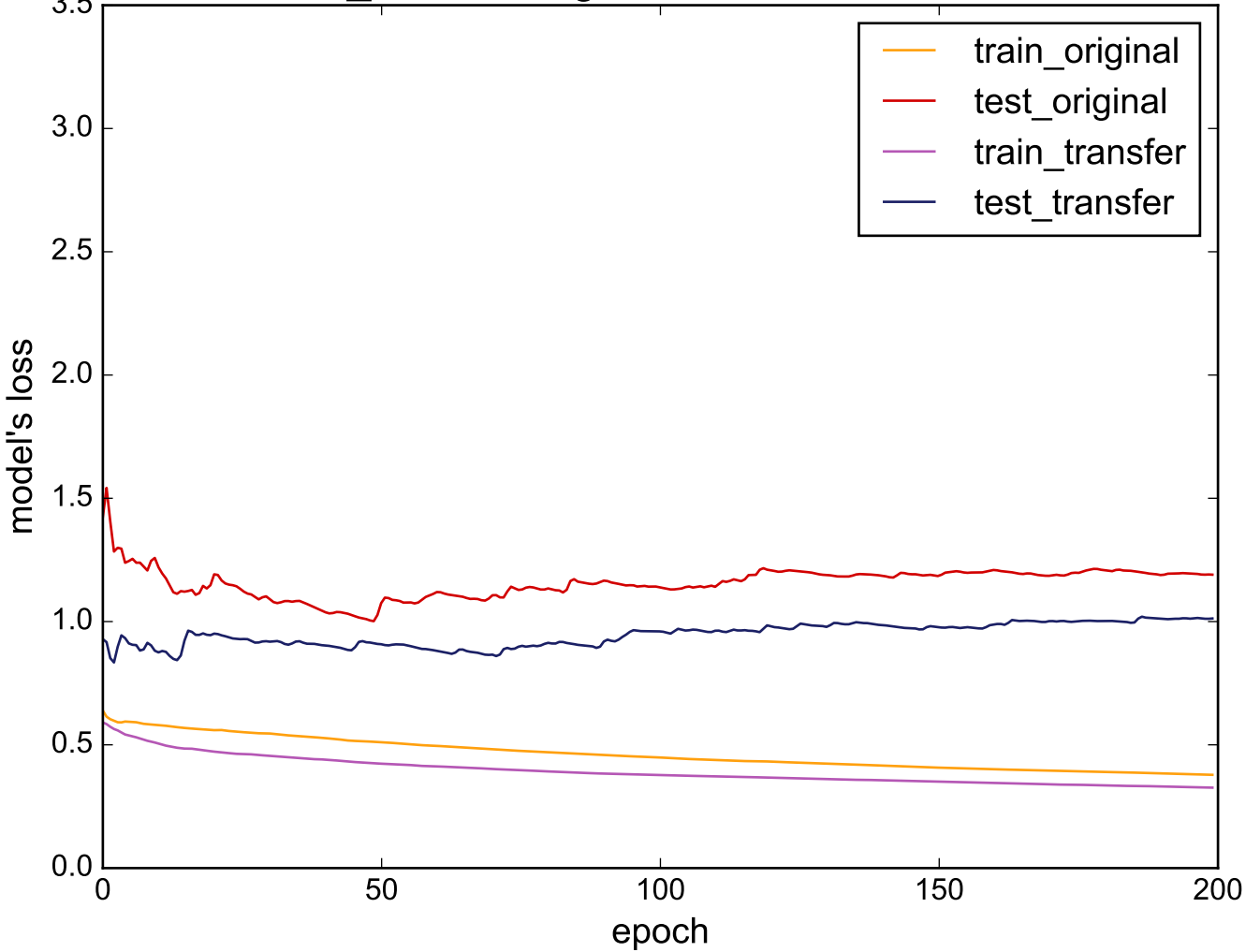
Source: Gun_Point - Target: MiddlePhalanxOutlineCorrect
