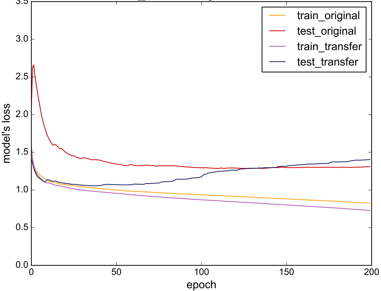
Source: Gun_Point - Target: MiddlePhalanxTW
