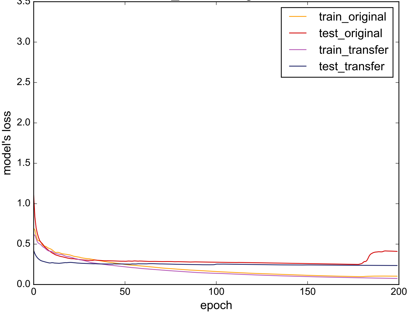
Source: Gun_Point - Target: MoteStrain
