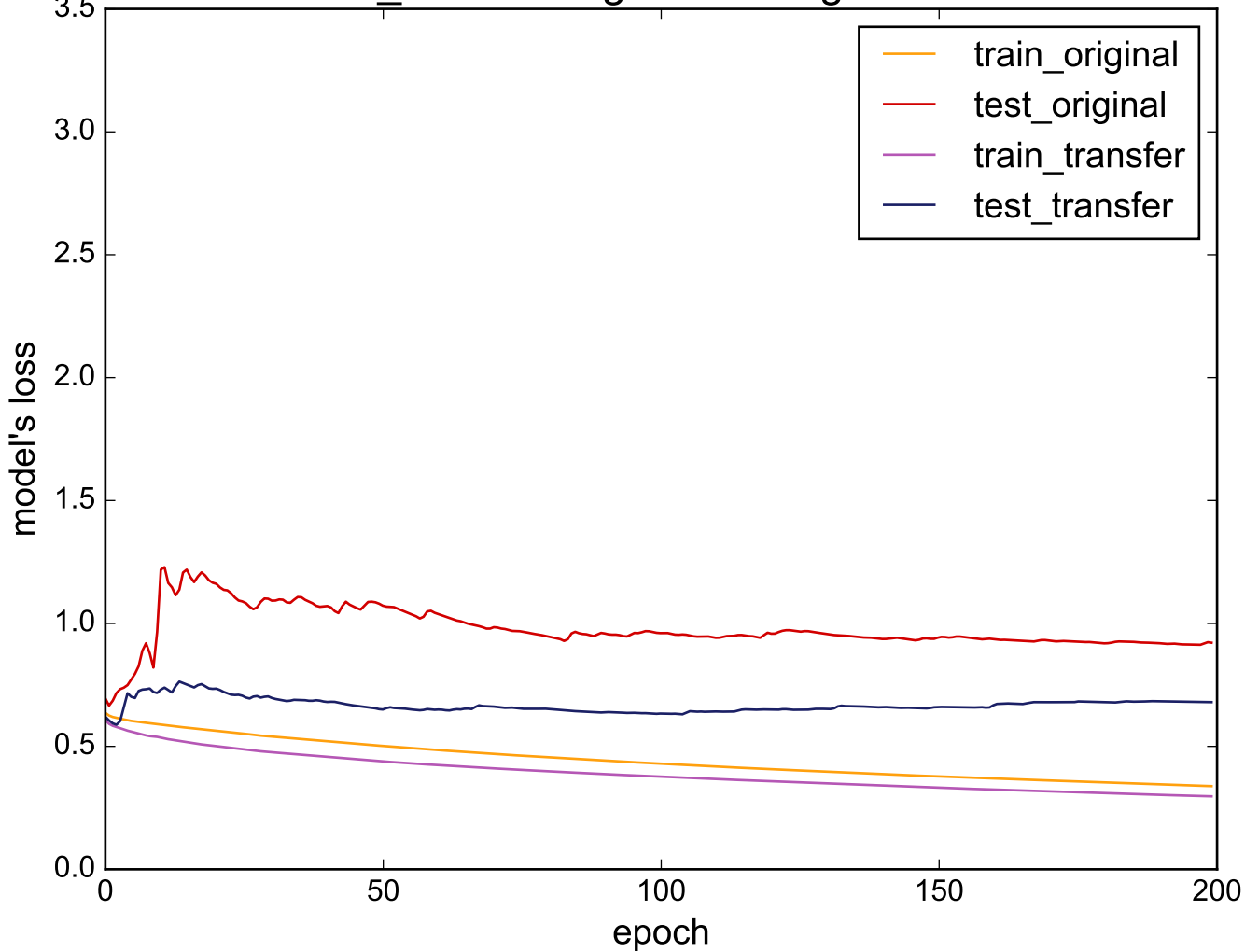
Source: Gun_Point - Target: PhalangesOutlinesCorrect
