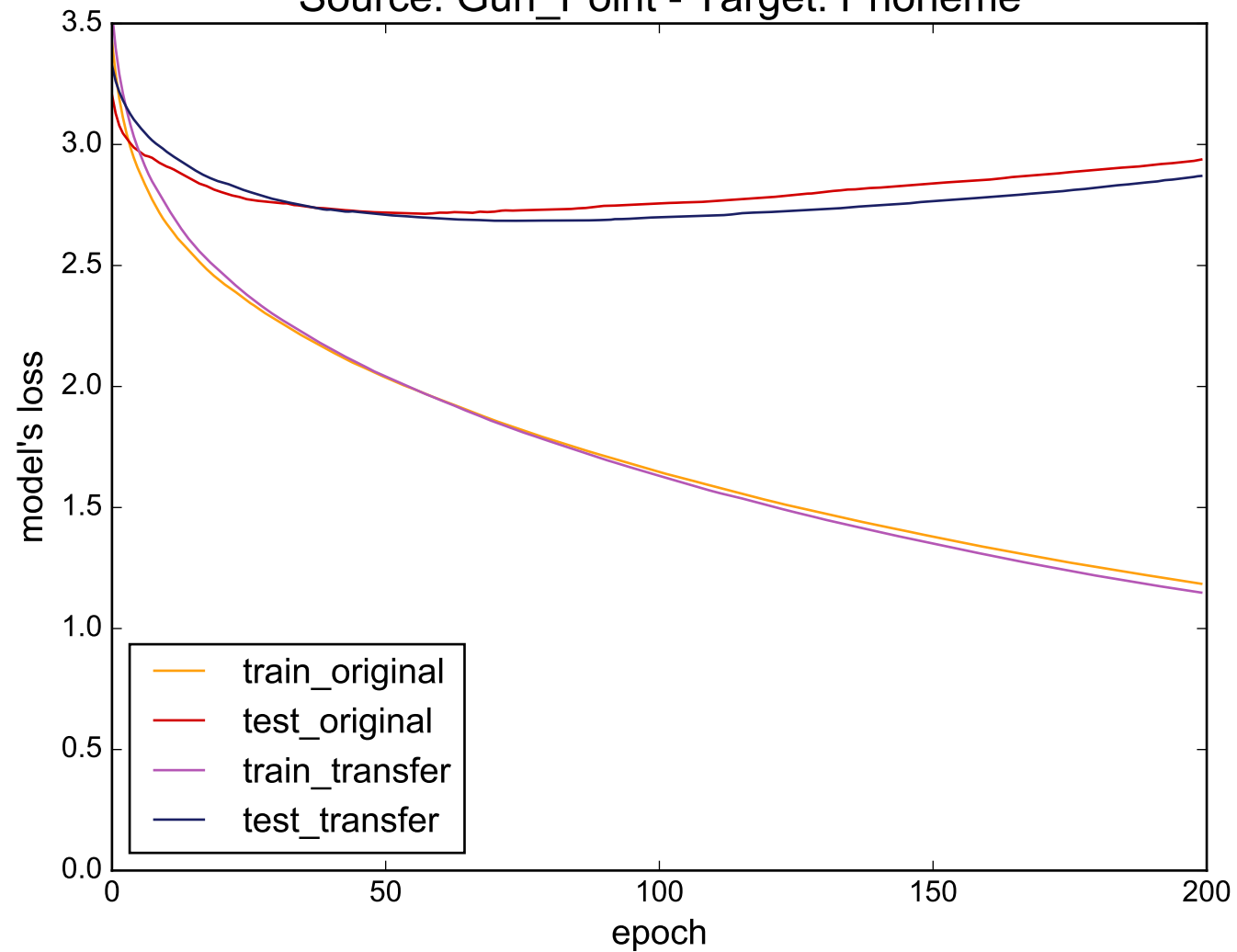
Source: Gun_Point - Target: Phoneme
