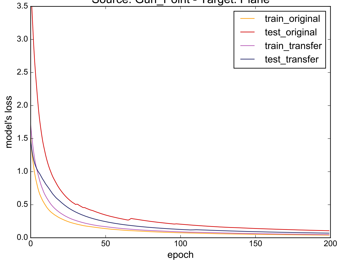
Source: Gun_Point - Target: Plane
