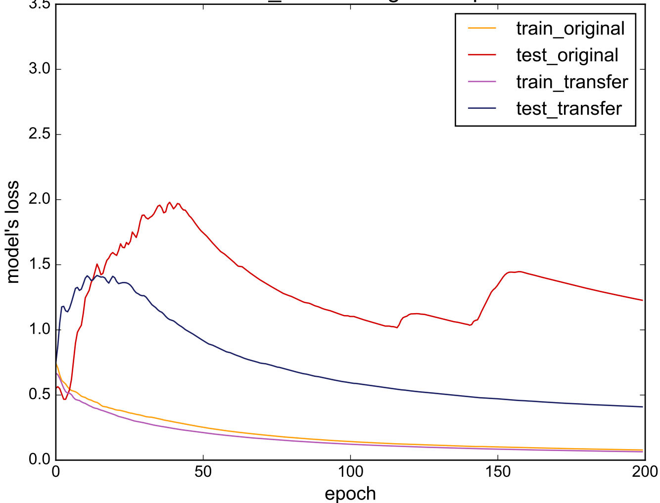
Source: Gun_Point - Target: ShapeletSim
