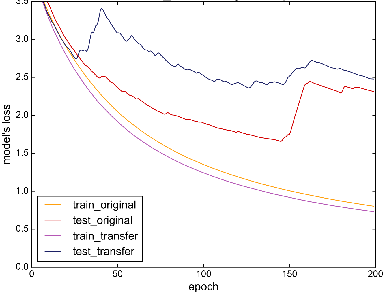
Source: Gun_Point - Target: ShapesAll
