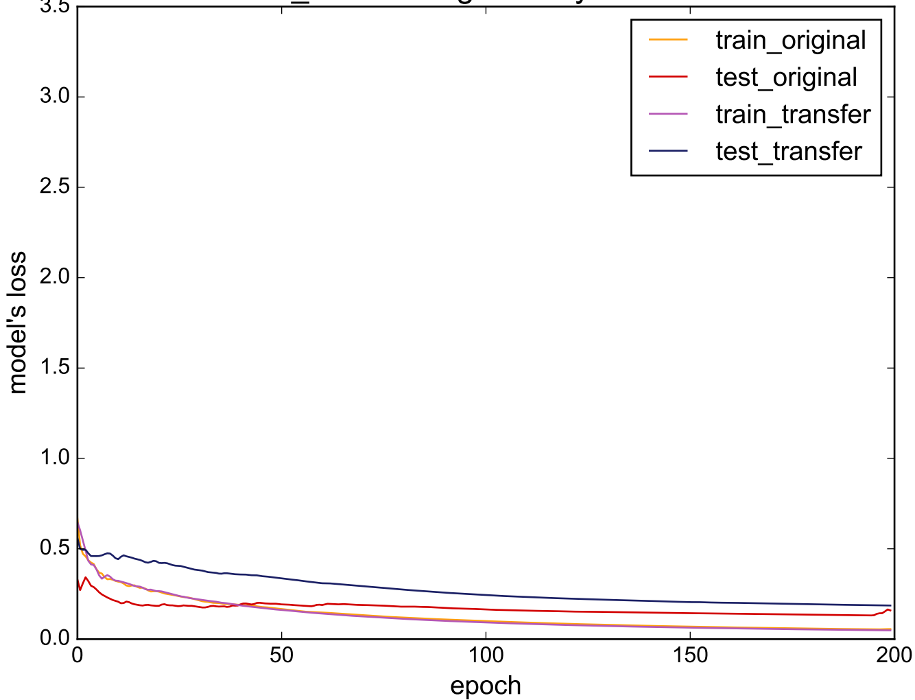
Source: Gun_Point - Target: SonyAIBORobotSurface
