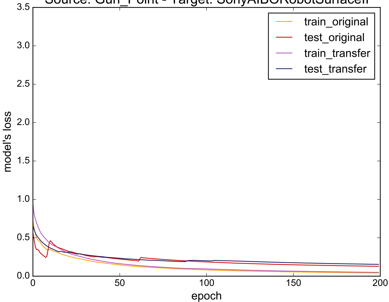
Source: Gun_Point - Target: SonyAIBORobotSurfaceII
