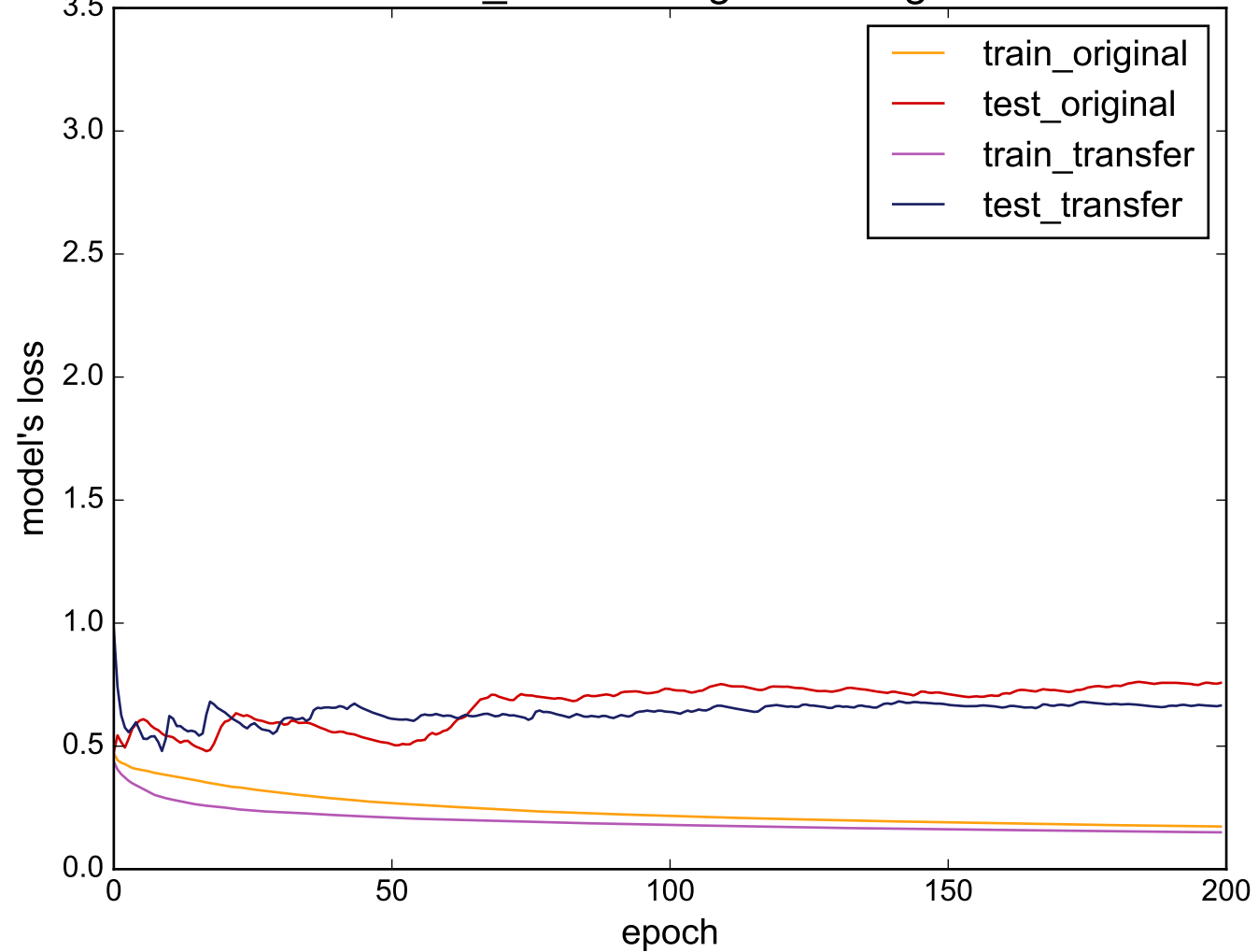
Source: Gun_Point - Target: StarLightCurves
