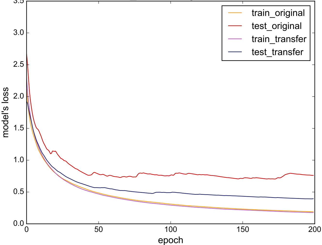
Source: Gun_Point - Target: SwedishLeaf
