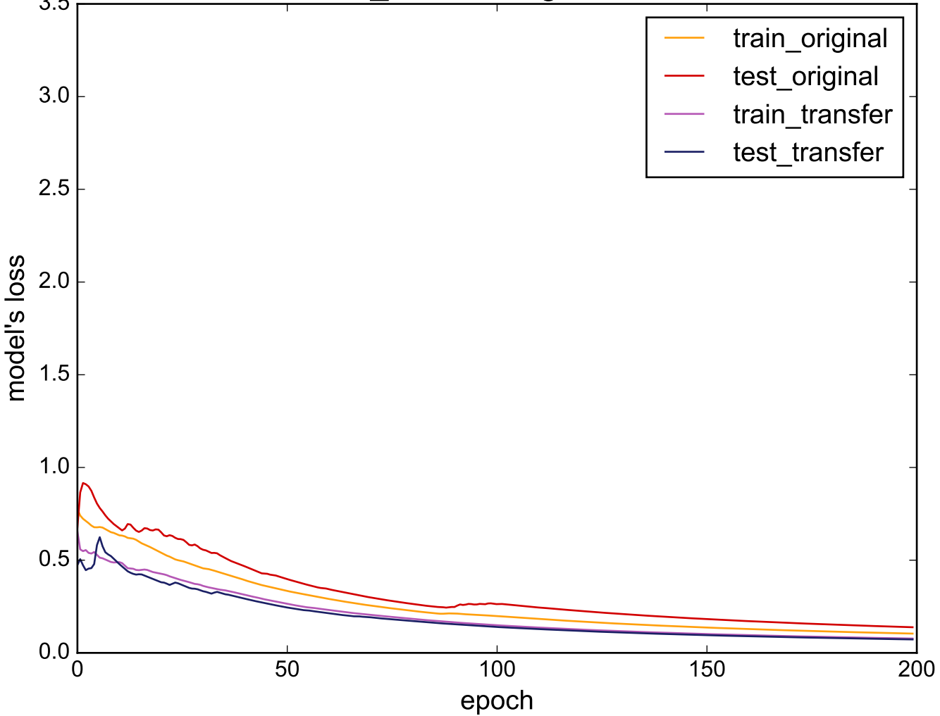
Source: Gun_Point - Target: TwoLeadECG
