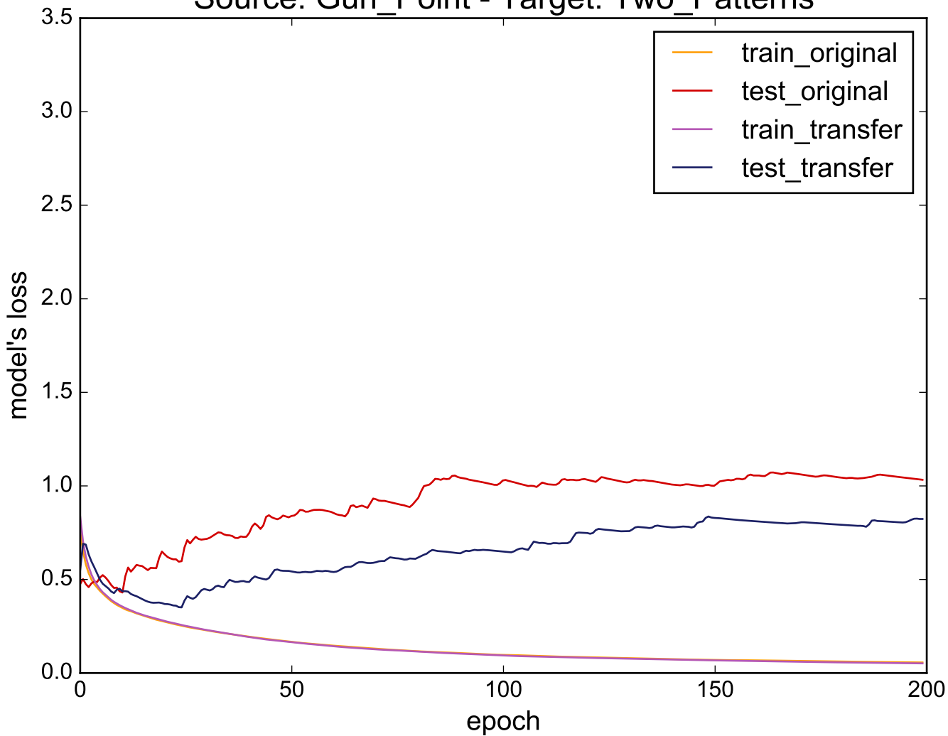
Source: Gun_Point - Target: Two_Patterns
