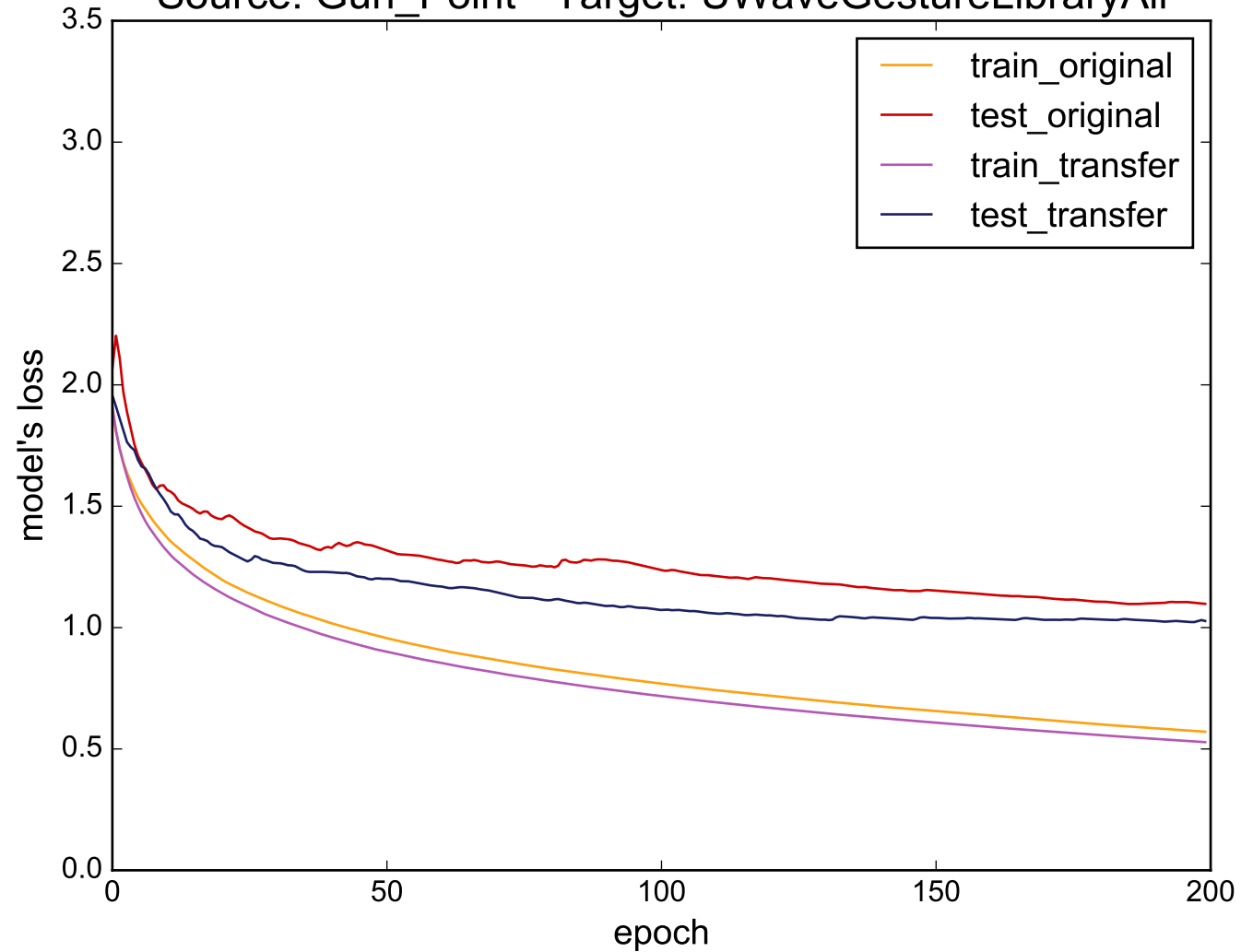
Source: Gun_Point - Target: UWaveGestureLibraryAll
