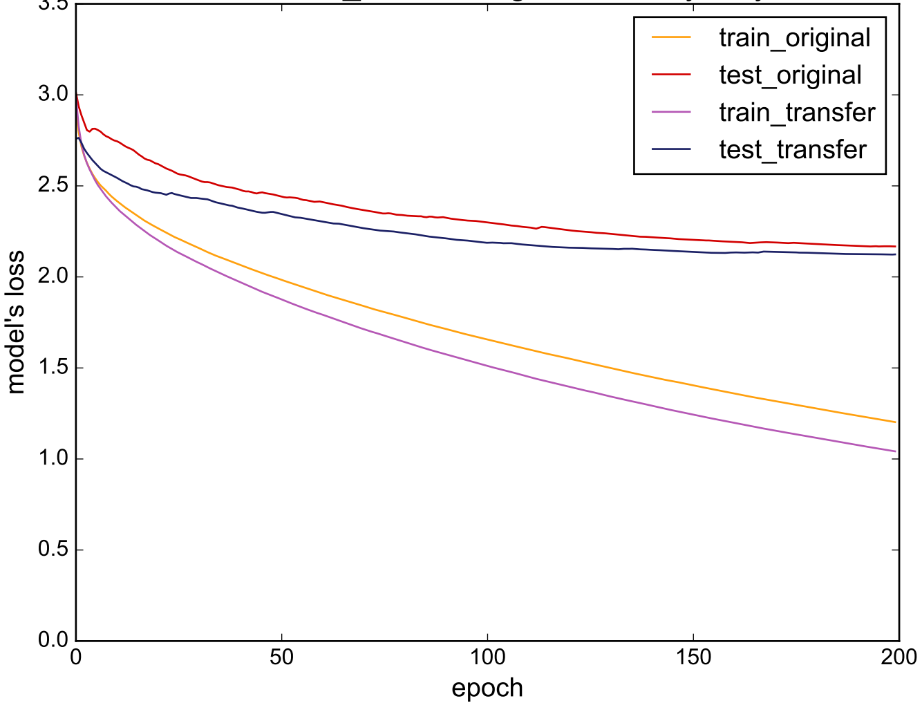
Source: Gun_Point - Target: WordsSynonyms
