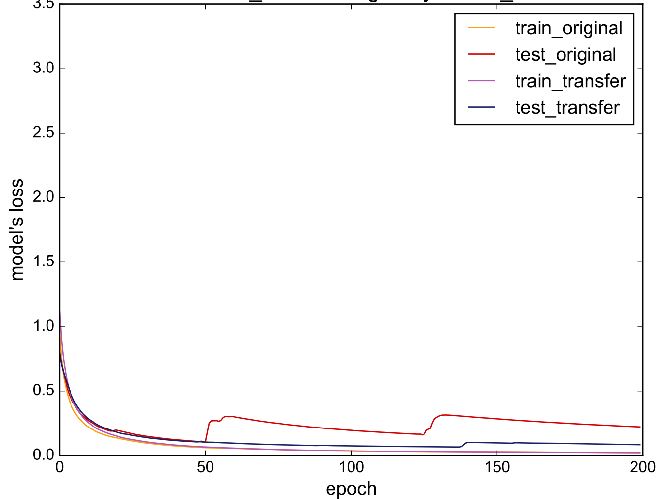
Source: Gun_Point - Target: synthetic_control
