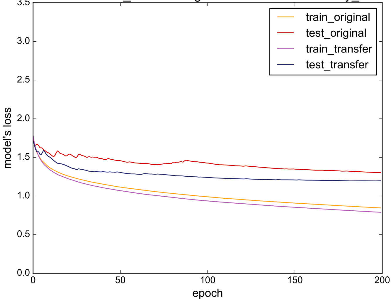
Source: Gun_Point - Target: uWaveGestureLibrary_Y
