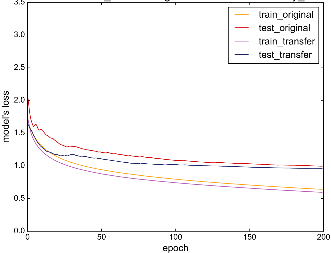
Source: Gun_Point - Target: uWaveGestureLibrary_Z
