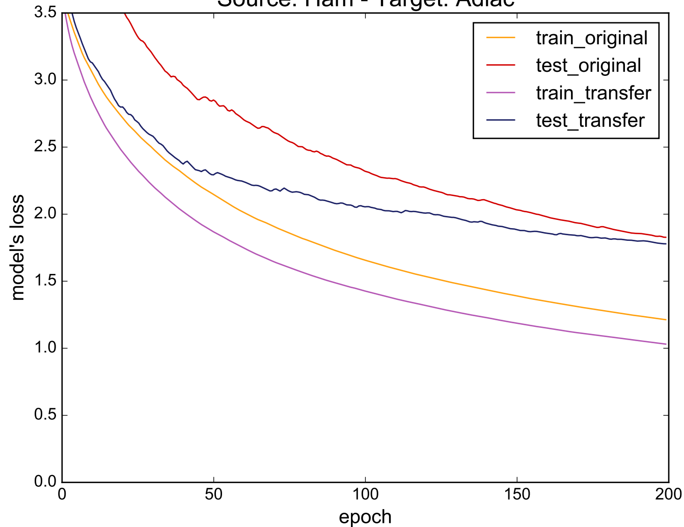
Source: Ham - Target: Adiac
