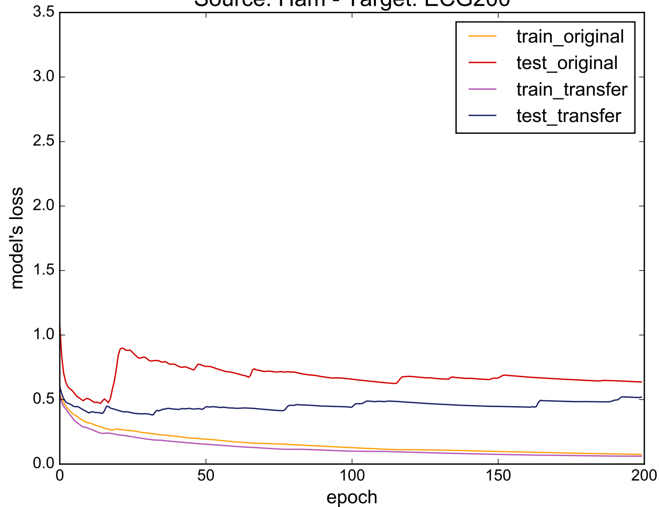
Source: Ham - Target: ECG200
