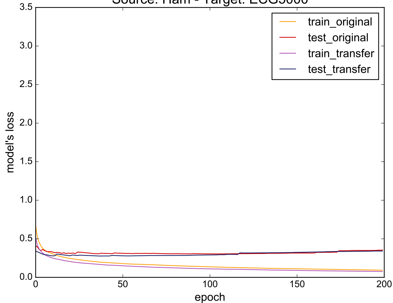
Source: Ham - Target: ECG5000
