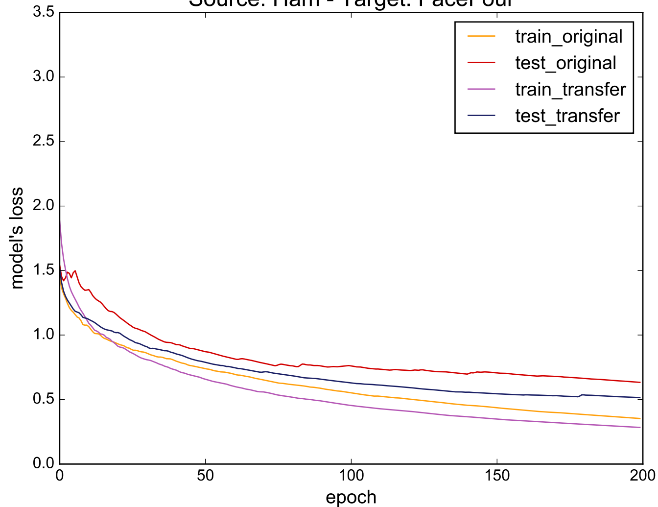
Source: Ham - Target: FaceFour
