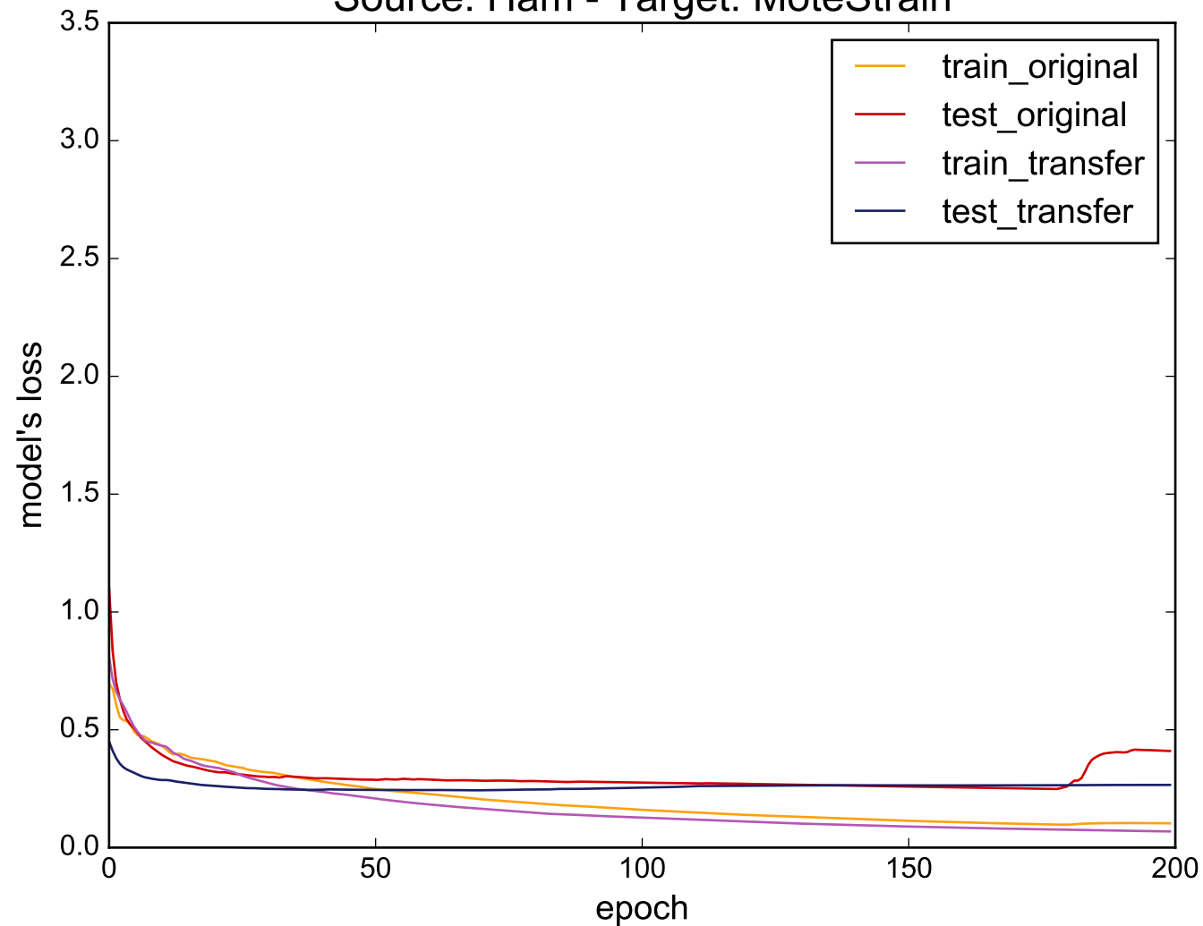
Source: Ham - Target: MoteStrain
