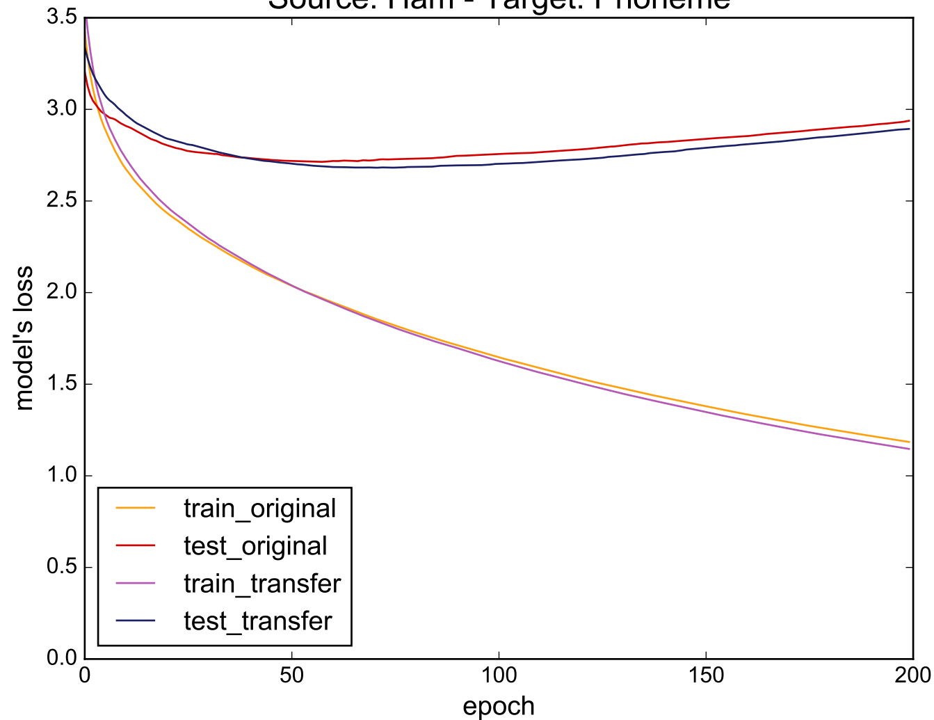
Source: Ham - Target: Phoneme
