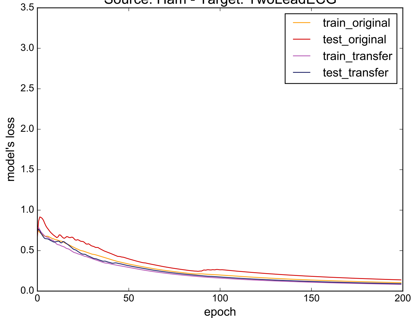
Source: Ham - Target: TwoLeadECG
