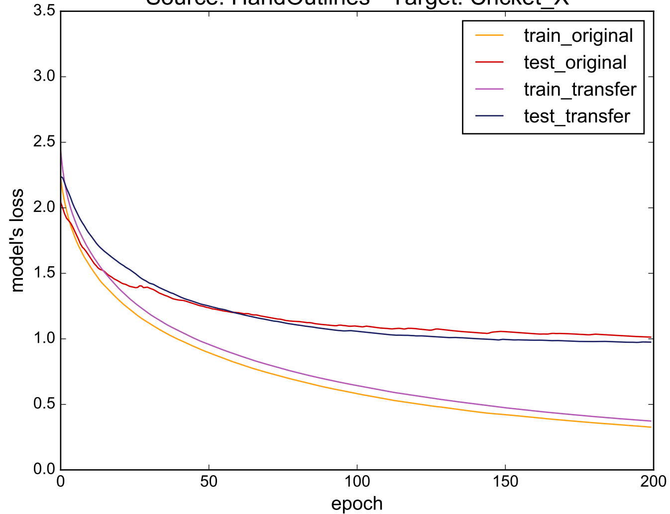
Source: HandOutlines - Target: Cricket_X
