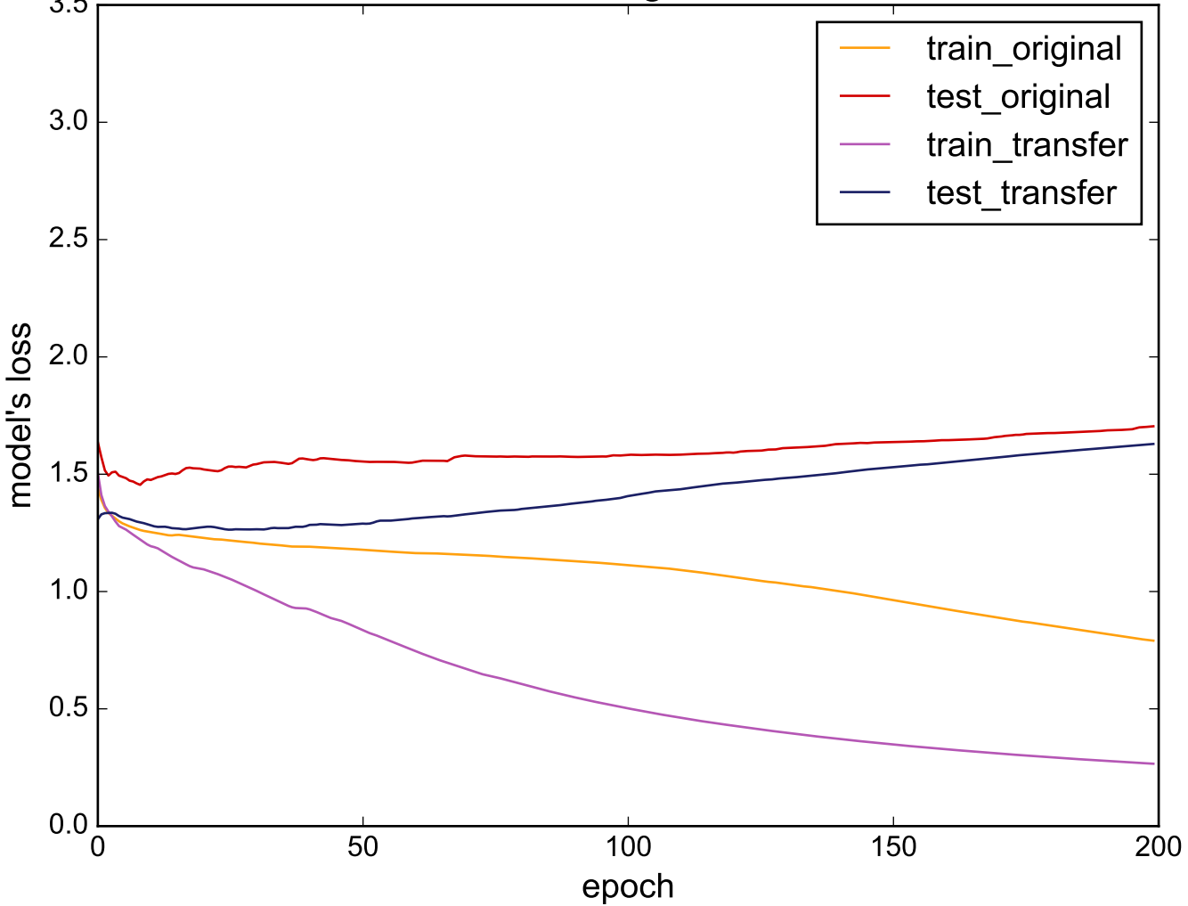
Source: HandOutlines - Target: DiatomSizeReduction
