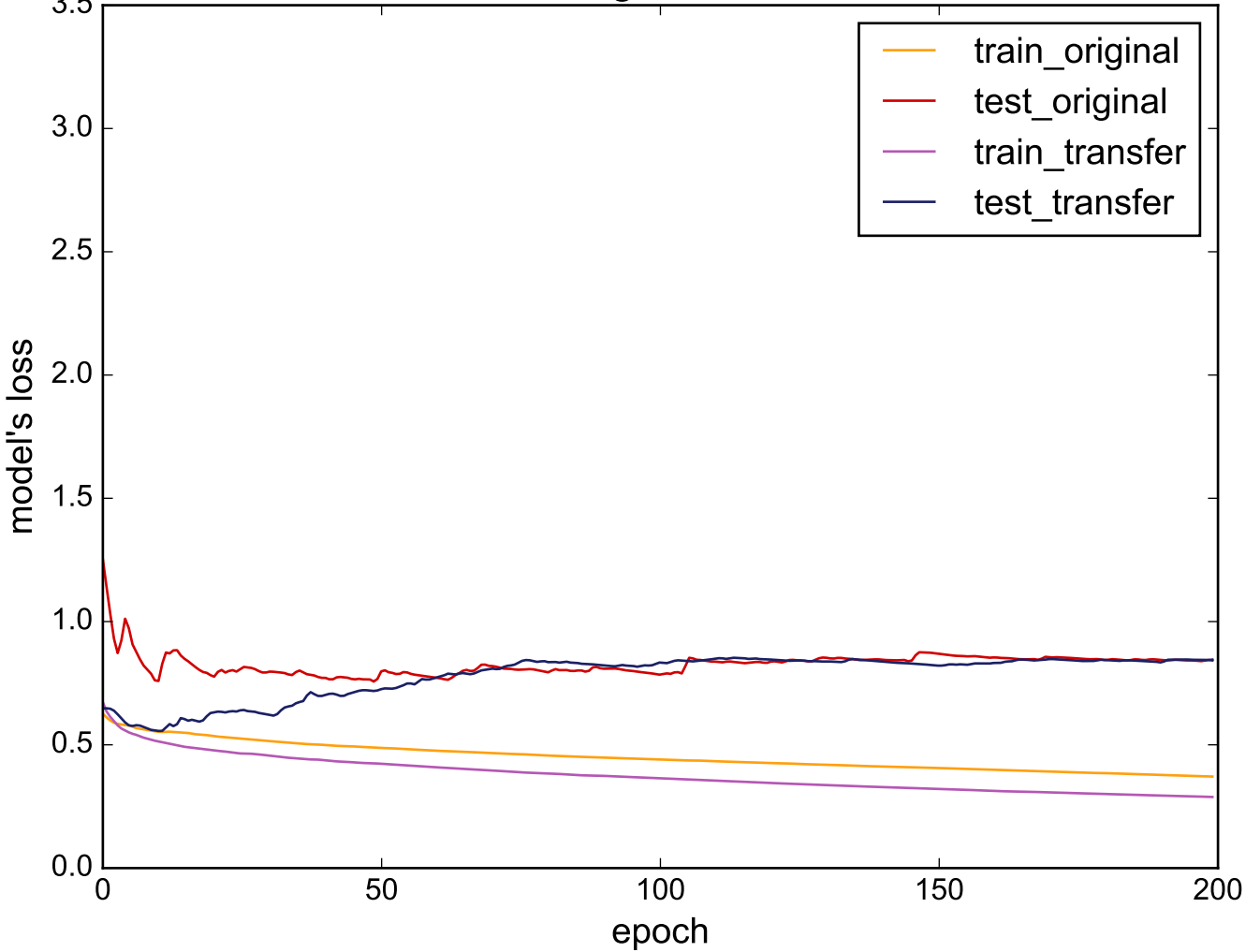
Source: HandOutlines - Target: DistalPhalanxOutlineCorrect
