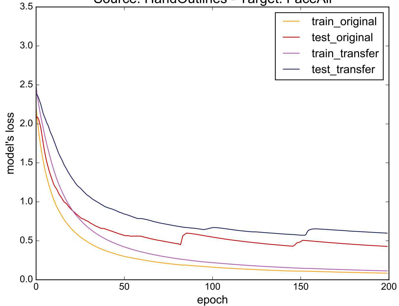
Source: HandOutlines - Target: FaceAll
