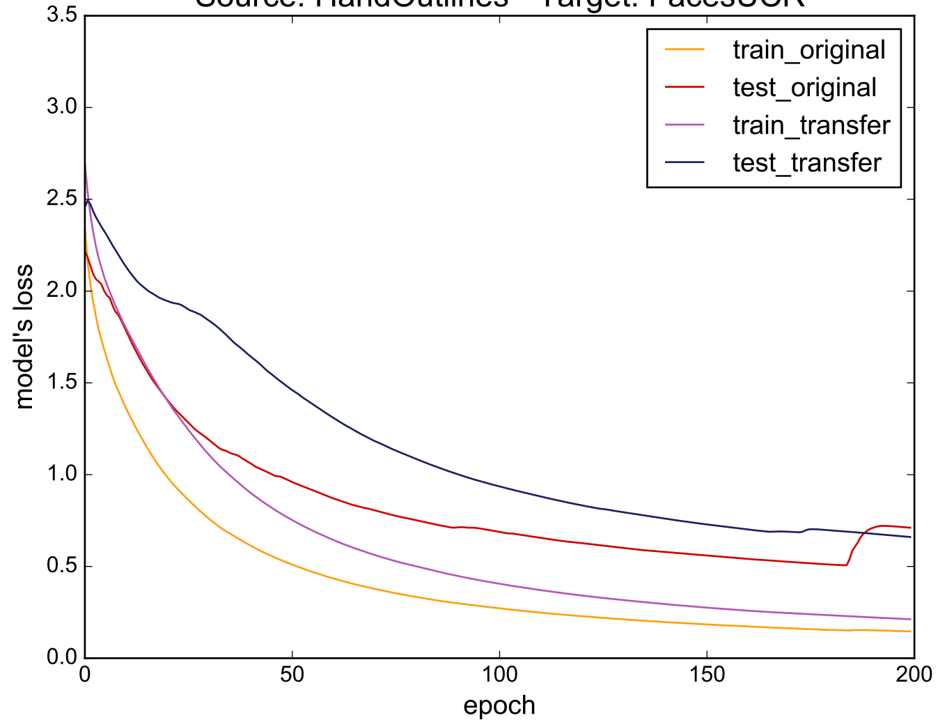
Source: HandOutlines - Target: FacesUCR
