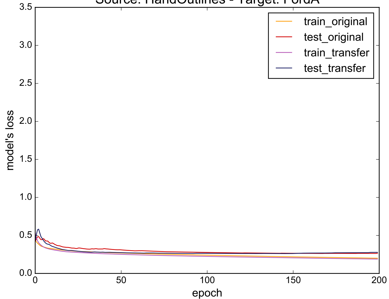
Source: HandOutlines - Target: FordA
