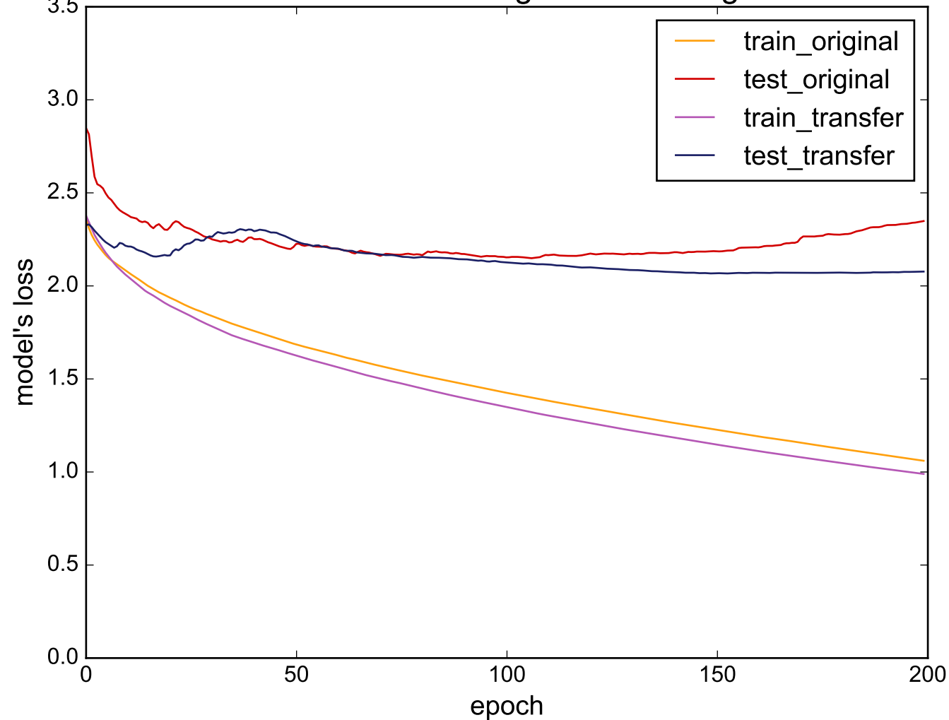
Source: HandOutlines - Target: InsectWingbeatSound
