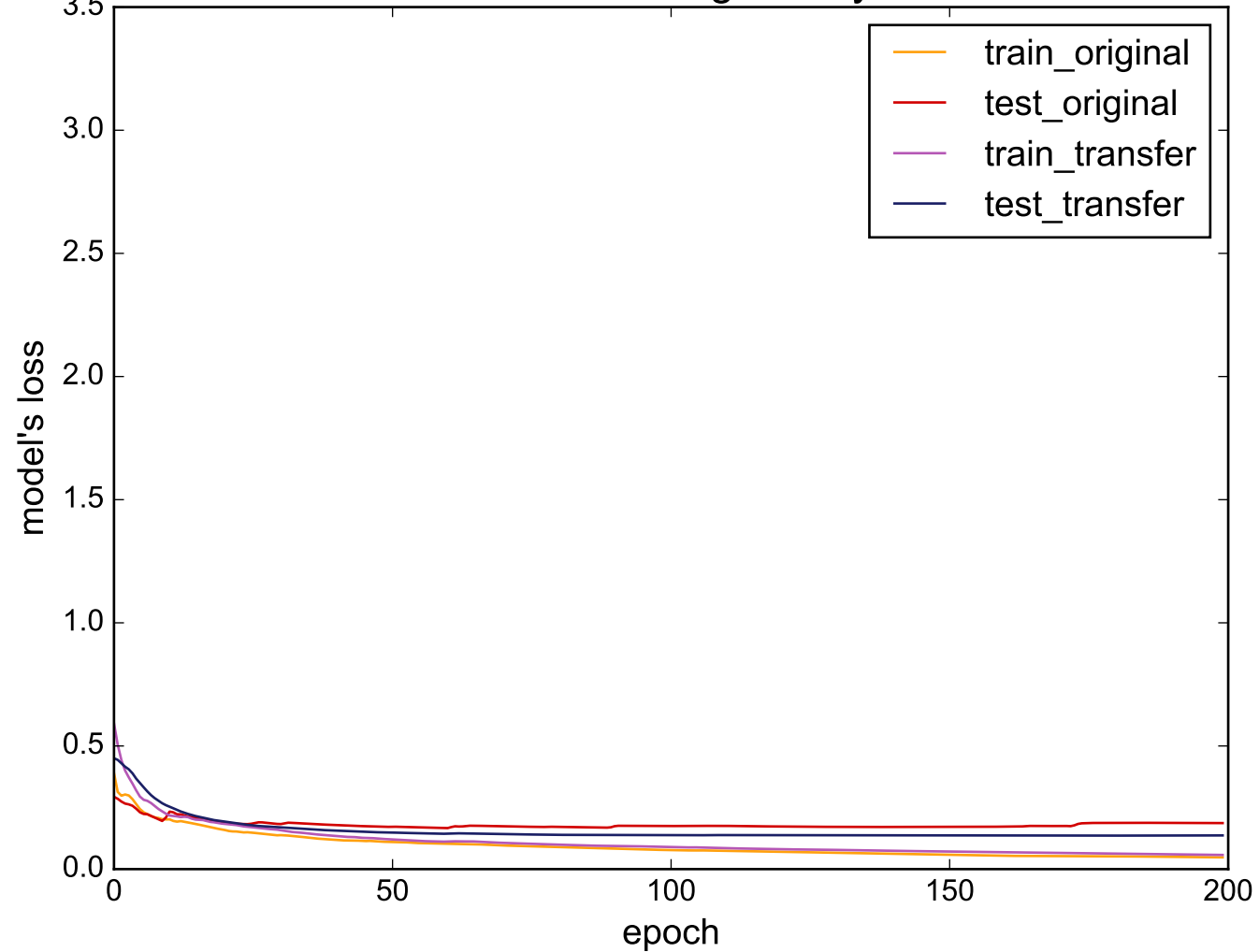
Source: HandOutlines - Target: ItalyPowerDemand
