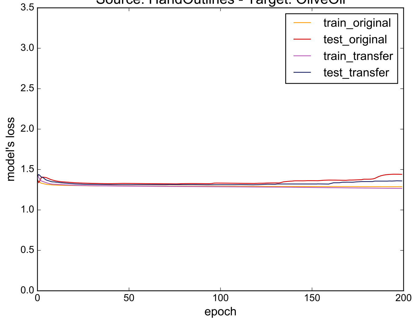
Source: HandOutlines - Target: OliveOil
