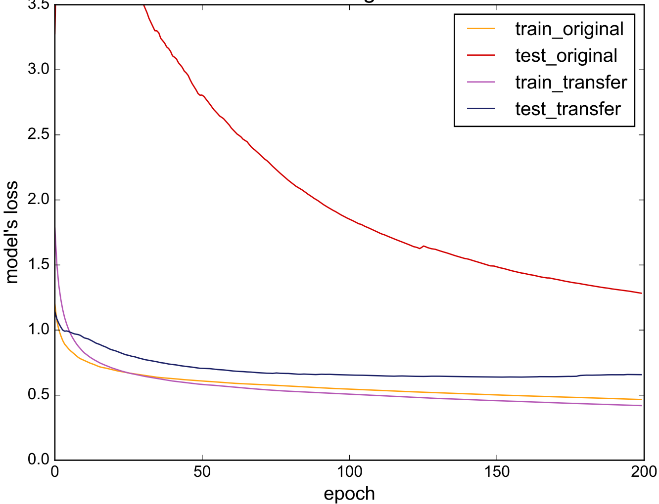
Source: HandOutlines - Target: ProximalPhalanxTW
