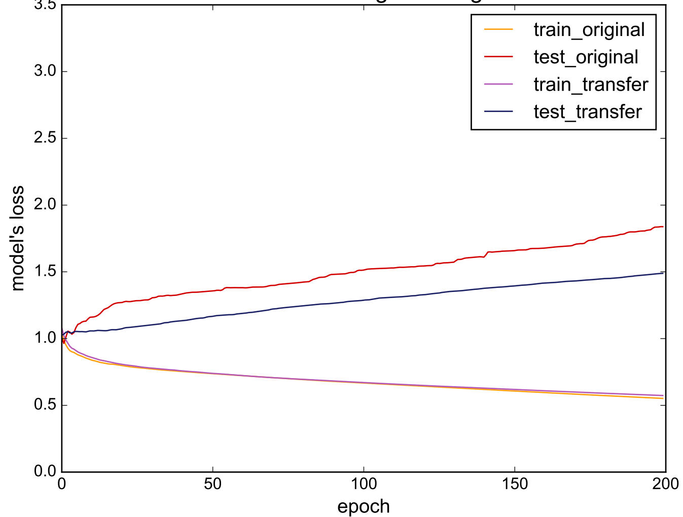
Source: HandOutlines - Target: RefrigerationDevices
