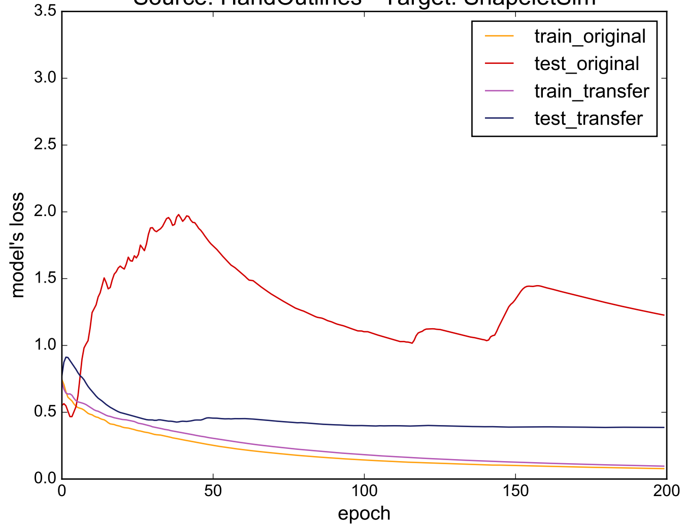
Source: HandOutlines - Target: ShapeletSim
