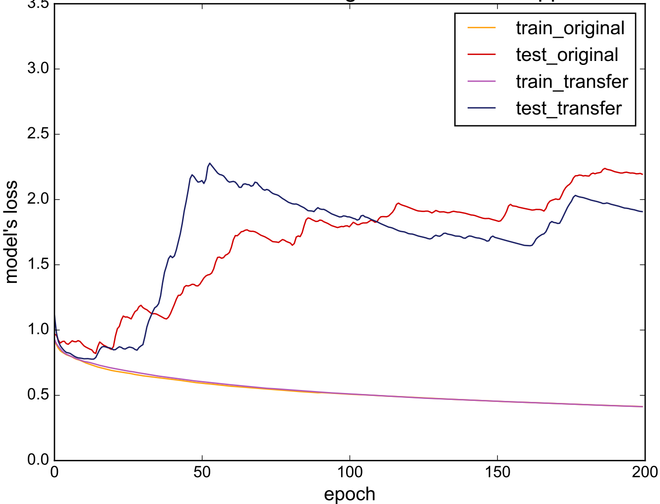
Source: HandOutlines - Target: SmallKitchenAppliances
