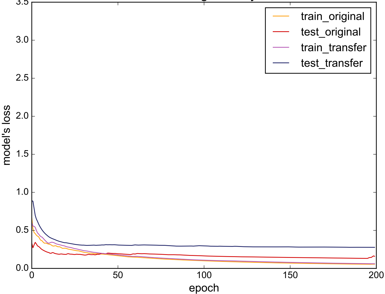
Source: HandOutlines - Target: SonyAIBORobotSurface
