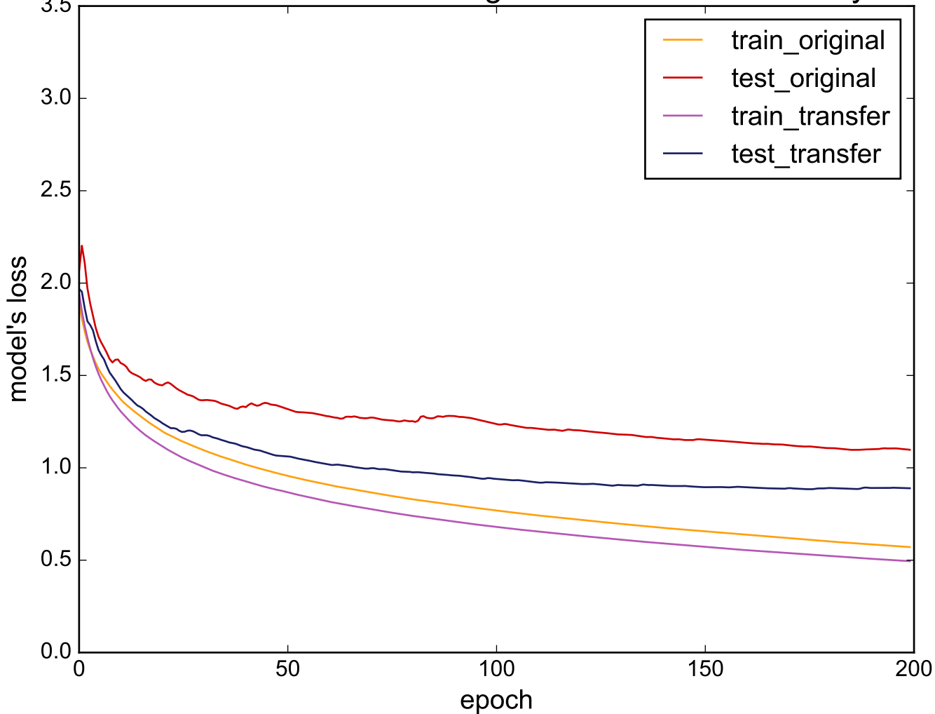
Source: HandOutlines - Target: UWaveGestureLibraryAll
